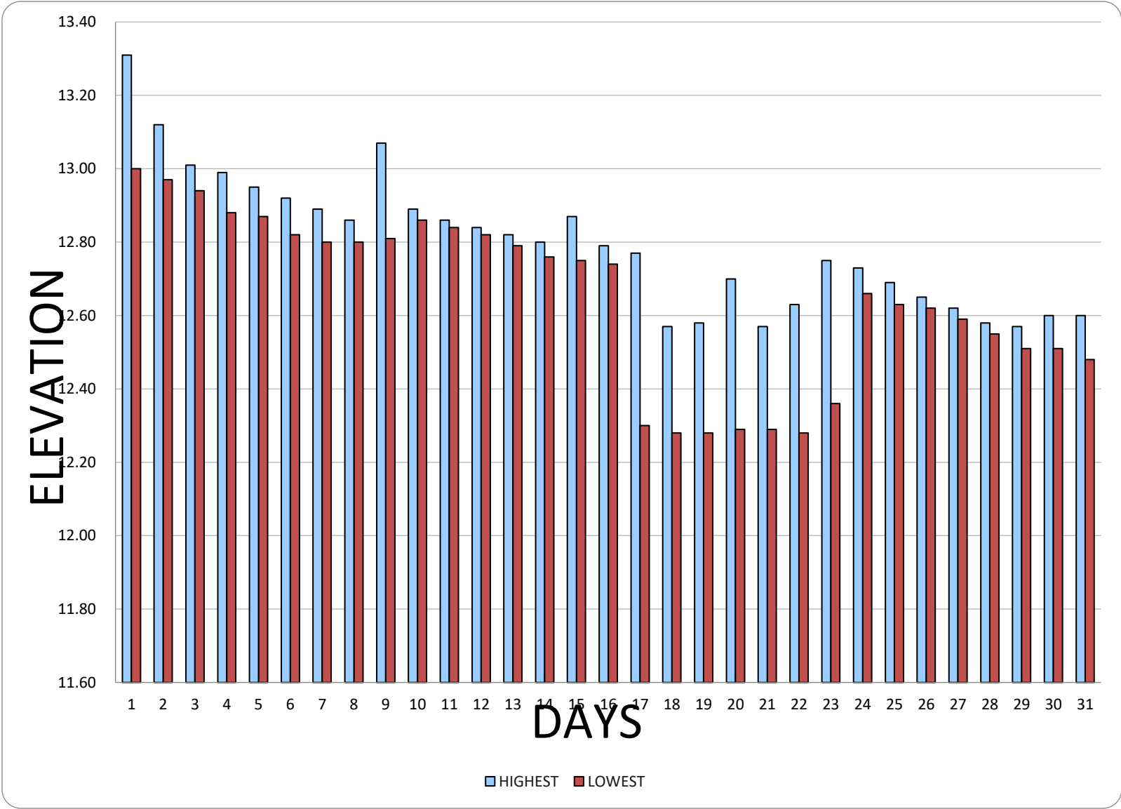
RECORDED DAILY HIGHEST AND LOWEST WATER ELEVATION STO. NINO WATER LEVEL GAUGING STATION December 1-31. 2025
